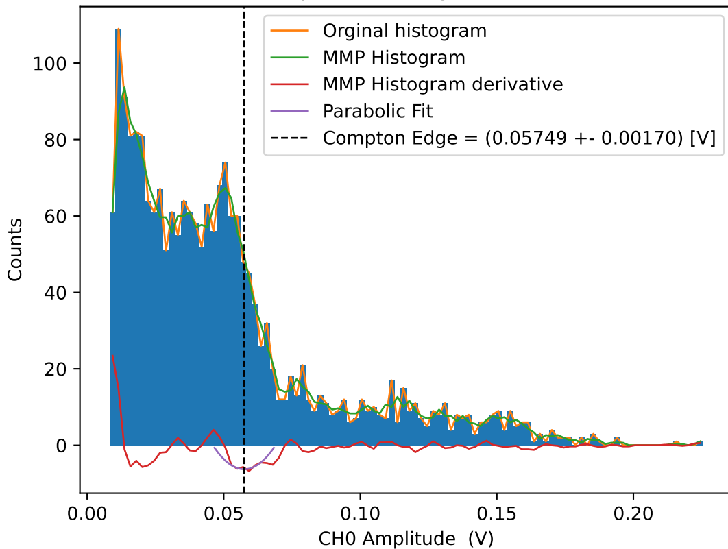
CH0 Amplitude histogram for 44.5V
